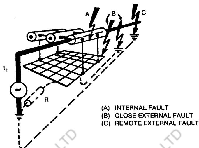
Figure 16—Typical faults in GIS
