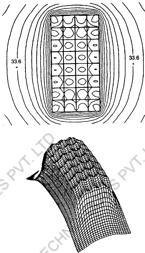
Figure 3—Equipotential contours of a typical grounding grid with and without ground rods
