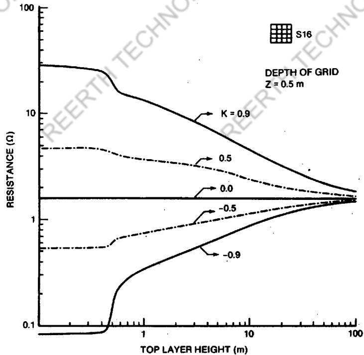
Figure F.4—Sixteen mesh grid resistance
